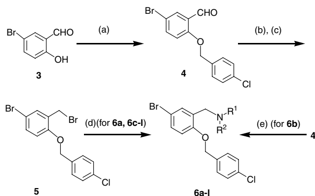
Scheme 1. Preparation of benzyl amine. Reagents and conditions: (a) 4-chlorobenzyl chloride, K 2 CO 3 , DMF, 120 °C, 4 h, 98%; (b) NaBH 4 , MeOH, rt; (c) CBr 4 , PPh 3 , CH 2 Cl 2 , 79% (two steps from 4 ); (d) R 1 R 2 NH, K 2 CO 3 , DMF, rt; (e) EtNH 2 , NaBH(OAc) 3 , CH 2 Cl 2 , rt, overnight.
