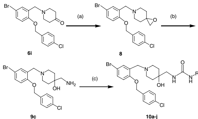
Scheme 2. Preparation of urea analogs. Reagents and conditions: (a) Me 3 S + I − , KO t Bu, DMSO, rt, 6 h, 94%; (b) in sealed tube, NH 4 OH, MeOH, 60 °C, 5 h, 81%; (c) RNCO, CH 2 Cl 2 , Et 3 N, rt, 2 h.
